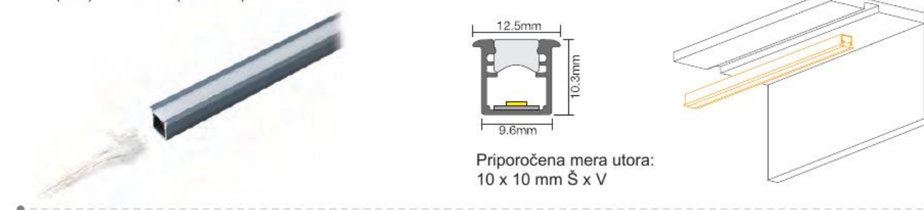
QC08A vgradna svetilka 12V (150)LED & 24V(200LED)-10W-CRI 90+
