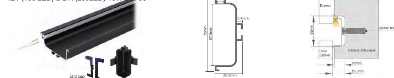
QC08B LED svetilka osvetlitev kabineta 12V (150 LED) & 24V(200LED)-10W-CRI 90+
