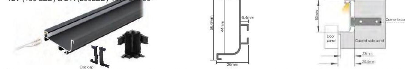
QC08B LED svetilka osvetlitev kabineta 12V (150 LED) & 24V(200LED)-10W-CRI 90+
