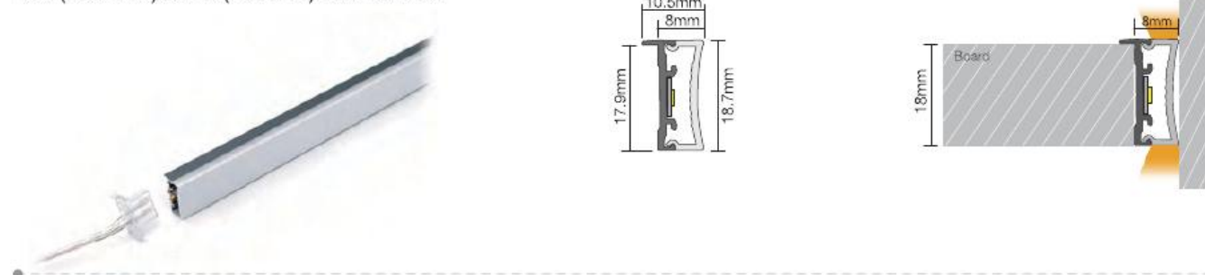
QC02A osvetlitev lesenih polic 12V (150 LED) & 24V(200LED)-10W-CRI 90+
